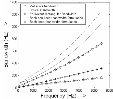
Fig. 2 – Bandwidth of the filters as against the centre frequency ( Hz) for the (a) Mel scale (b) Critical Bandwidth (c) Equivalent rectangular Bandwidth (d) 'Bach' Non-linear scale, (e) 'Bach' linear scale
