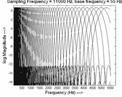
Fig. 3 – The Bach scale Filter-bank Non-linear case
